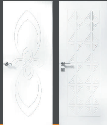
Model Personalization
